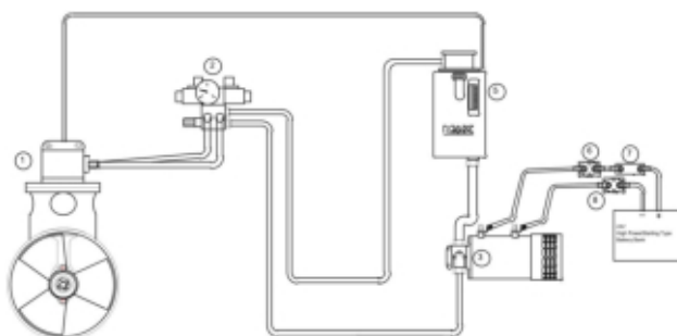
1. Hydraulic Motor & Thruster 2. Service Valve (DCV) 3. Electro-Hydraulic Pump (EHP) 4. Check Valve 5. Hydraulic Oil Reservoir with Filtration System 6. Electric/Manual Battery Isolator 7. Power Fuse 8. Power Relay
