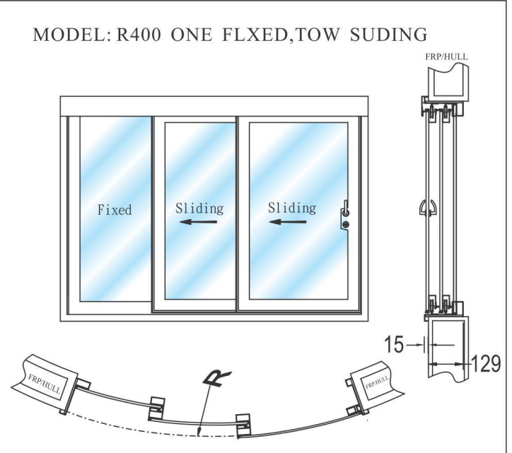
Screendoor(two sliding)
