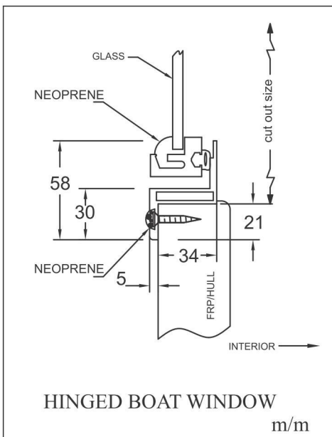
HINGED BOAT WINDOW
