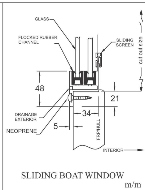
SLIDING BOAT WINDOW
