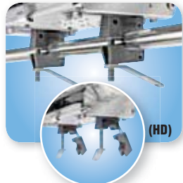
"Dual" Horizontal Round Rail Mount T10-580 Standard Rails 7/8" or 1" (22 mm or 25.5 mm) T10-585 Oversize Rails 1-1/8" or 1-1/4" (28.5 mm or 32 mm) T10-590 Large Rails 1-1/2" (38 mm) Fits all ChefsMate, Newport, Catalina & Monterey Grills & "DM" Tables
