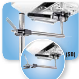
Vertical "LevelLock" Round Rail Mount T10-780 Standard Rails 7/8" or 1" (22 mm or 25.5 mm) T10-785 Oversize Rails 1-1/8" or 1-1/4" (28.5 mm or 32 mm) T10-790 Large Rails 1-1/2" (38 mm) Fits 12" x 18" or smaller rectangular grills and "SM" tables
