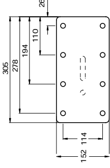
Baseplate S225, S225 Tall, S250, S250 Tall, S300
